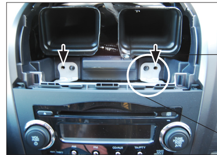
5. Remove the two screws above the OEM head unit
