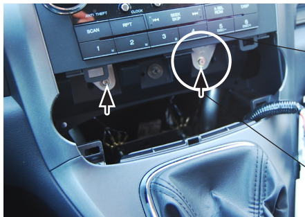
3. Remove the two screws below the OEM head unit
